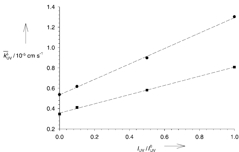
Figure 4. Dependence of \bar{k}_{UV}^{\delta} on UV irradiation intensity at 670 °C for final P_{O_2} values of 0.08 (circles) and 0.02 bar (squares). I_{UV}^0 is the full UV intensity; I_{UV} is the intensity attenuated by neutral density filters.
